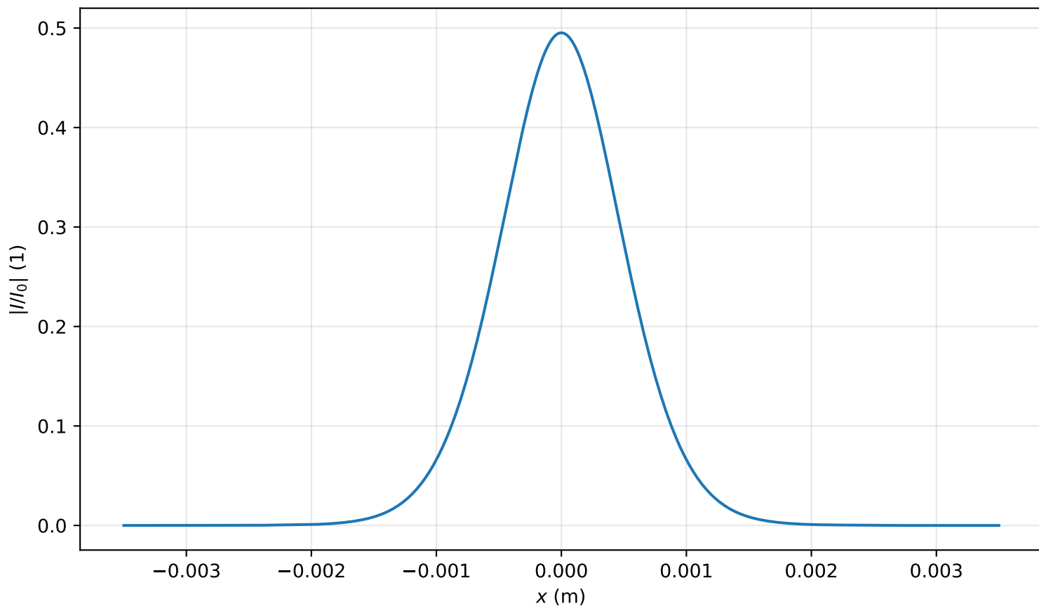
Intensity profile I(x, y = 0, z = 2.946m)/I_0 , P_{in}=0.4P_{cr} , artificial time
